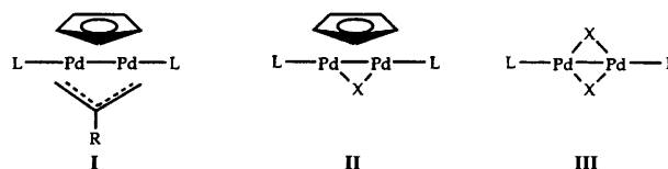
Scheme 1 Examples of \text{Pd}^{\text{I}}\text{-Pd}^{\text{I}} dimers with: two organic bridging groups ( I ), one organic bridge and one halogen ( II ) and two bridging halogens ( III ) (L = phosphine; R = H or alkyl; X = Cl, Br or I)
