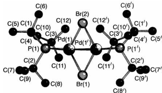
Fig. 1 Molecular structure of [\text{Pd}_2(\mu\text{-Br})_2(\text{PBU}_3)_2] . Important bond lengths (Å) include: Pd(1)–Pd(1') 2.628(2), Pd(1)–Br(2) 2.460(4), Pd(1)–P(1) 2.296(4) [distances for the second half molecule: Pd(2)–Pd(2') 2.621(2), Pd(2)–Br(3) 2.454(4), Pd(2)–P(2) 2.303(4)]
